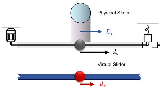
Fig. 4. Displacements during interaction: D_r , Displacement of the robotic arm with regard to physical world; d_s , Displacement of the physical slider knob with regard to the slider itself; and d_v , Displacement of the virtual slider knob with regard to the virtual world.
