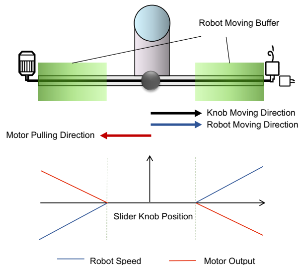
Fig. 5. Interaction scenario for the dynamic slider. The robot arm moves in the same direction as the slider knob movement, while the slider motor is pulling in the opposite direction. As the knob gets close to the end of the slider, the speed of the robotic arm and motor output increases.
