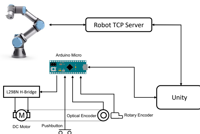
Fig. 3. System connection diagram. A TCP server is used for communication between robot and Unity, and an Arduino is used for communication between physical pops and Unity.
